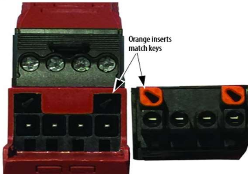
Figure 88 - Orange-colored Keyway
