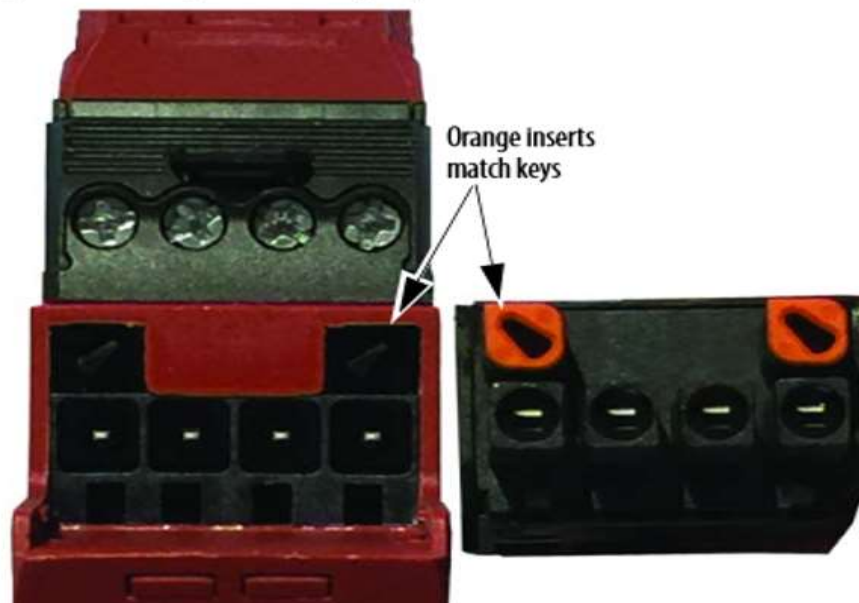
Figure 88 - Orange-colored Keyway
